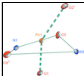
Fig. 2. \Psi -Monocapped octahedral geometry of lead. Symmetry codes are given in Table 1.
